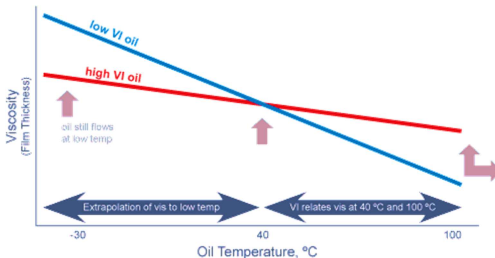
Figure 2. Oil viscosity vs. oil temperature.
